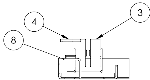
DETAIL D SCALE 1 : 4
